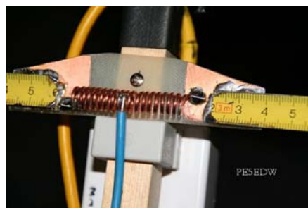
Reflector details
